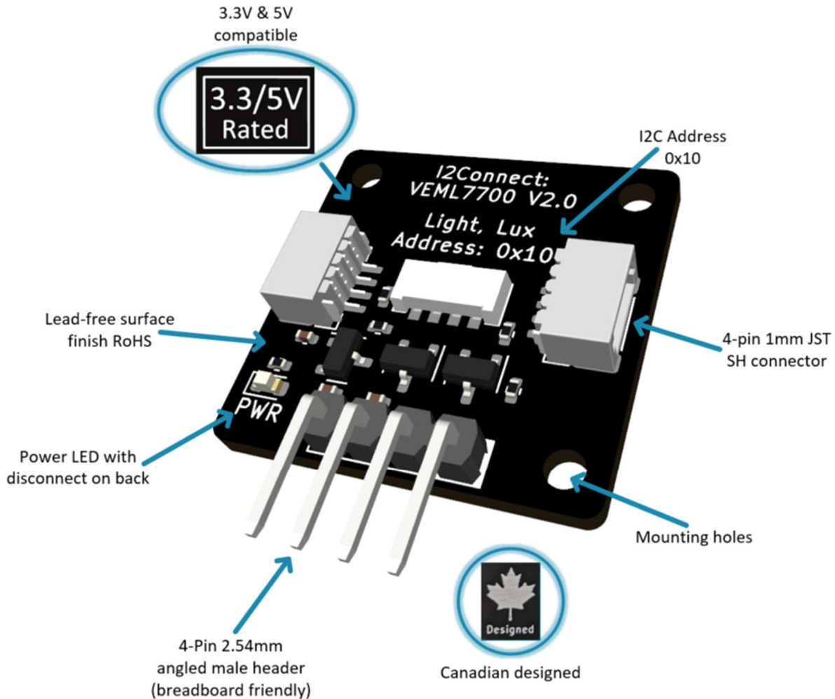
Figure 2: Technical Features Diagram for the I2Connect: VEML7700.
