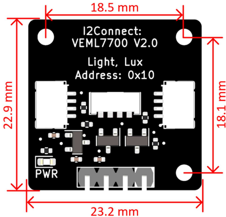
Figure 7: Dimensions of the I2Connect: VEML7700.
