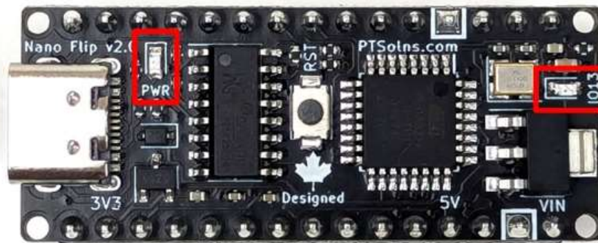
Figure 3: The power (PWR) and programmable (IO13) LEDs on the Nano Flip.
