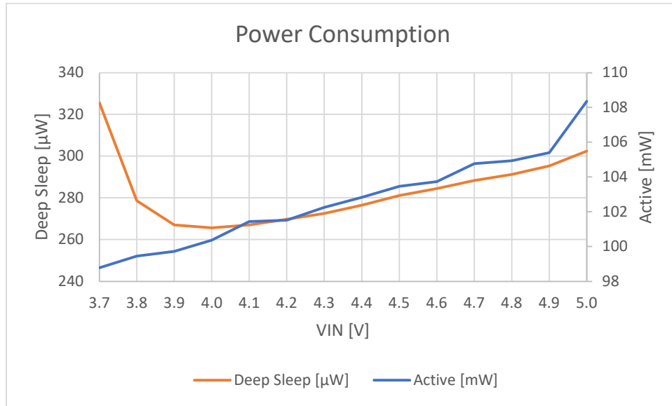
Figure 7: Power consumption of the ESP32 microWatt.
