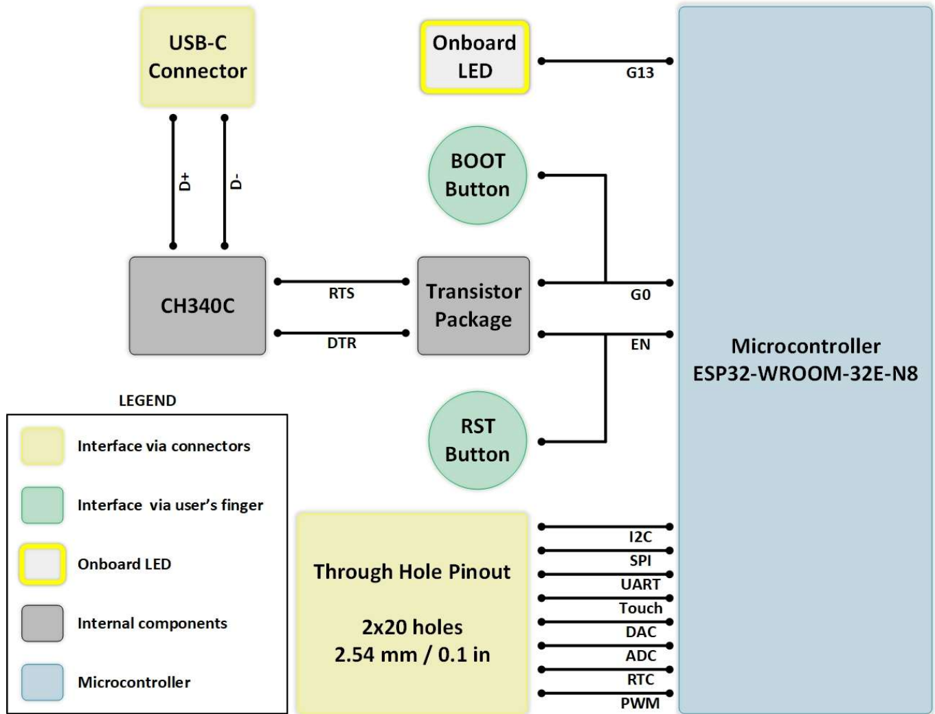
Figure 1: ESP32 microWatt Block Diagram.
